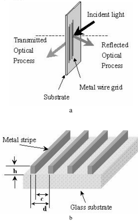
Fig. 1. (a) Schematic of the nanograting PBS, where TM polarized light is transmitted and TE polarized light is reflected. (b) Metal wire nanograting model.
