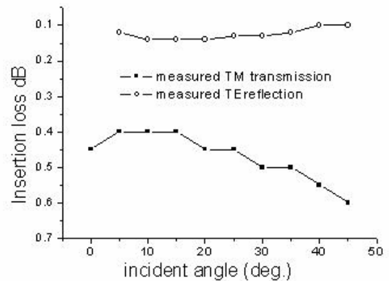
Fig. 8. Experimental result of insertion loss measured as a function of incident angle.
