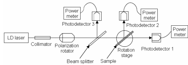
Fig. 7. Schematic diagram of the experimental setup for measurement of the efficiency of the embedded nanograting.
