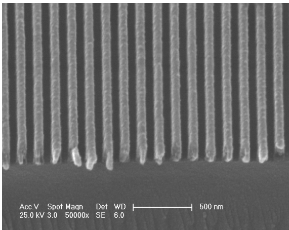
Fig. 5. Scanning electron microscope photographs of the grating sample with a period of 150 nm and a duty cycle of 0.5.
