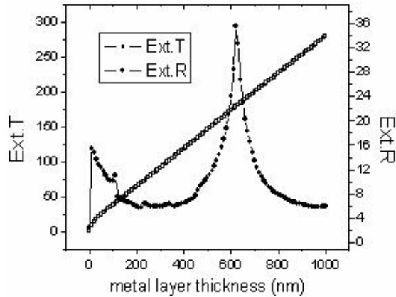
Fig. 3. Extinction ratio of transmission and reflection (Ext.T and Ext.R) as a function of metal layer thickness h .
