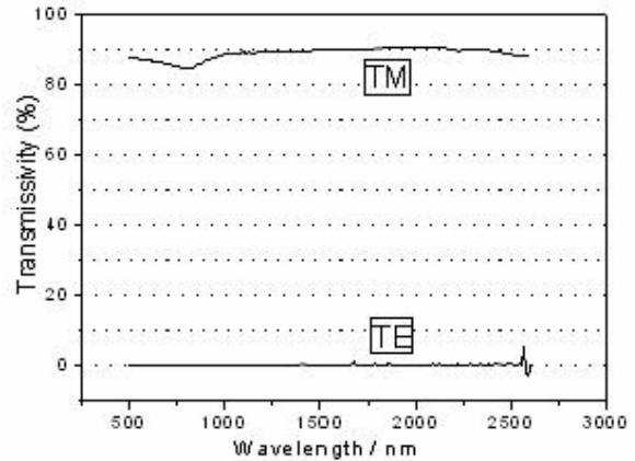
Fig. 6. Transmission spectrum measured for TE and TM wave.
